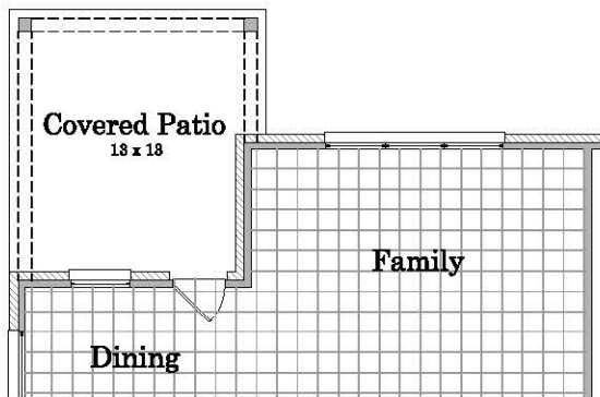
Extended Covered Patio Option
