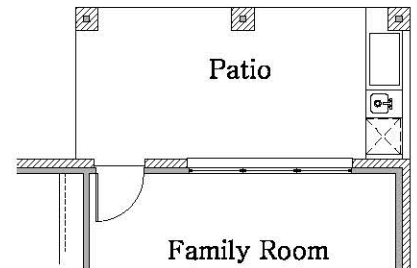
Outdoor Kitchen Option
