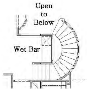
Wet Bar w/ Circular Staircase
