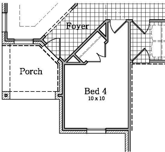
Bedroom 4 Option
