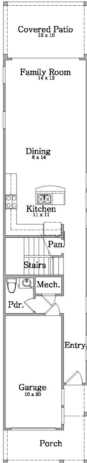
First Floor Plan - 1
